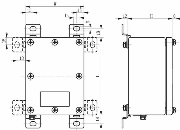
CZ1320 不锈钢接线箱 (开盖式) Stainless steel terminal box (Cover-open type)
