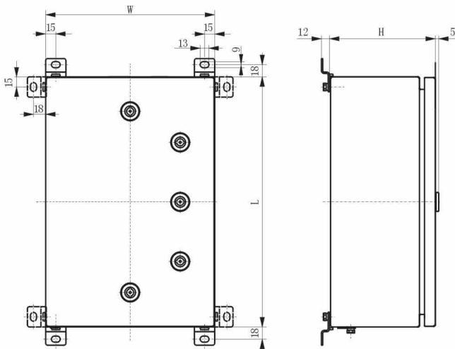
CZ1320 不锈钢接线箱 (开门式) Stainless steel terminal box (Door-open type)
