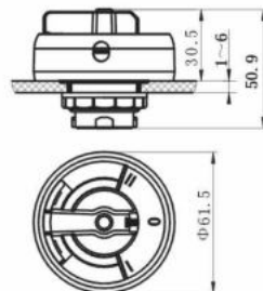
CZ4000-SE4 防爆开关操作头 Operation head of explosion-proof switch
