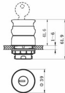
CZ4000-Y2E 防爆(急停)钥匙释放按钮操作头 Operation head of explosion-proof (emergency stop) key-releasing push button
