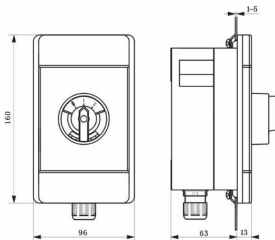
CZ0240/9-□-□ 面板式安装防爆按钮、开关 (4P) Explosion-proof push button, switch for panel mounting (4P)
