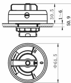
CZ4000-SE4 防爆开关操作头 CZ4000-SB4 防爆开关操作头 Operation head of explosion-proof switch
