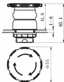
CZ4000-P7E 防爆(急停)扭动释放按钮操作头 CZ4000-P7B 防爆(急停)扭动释放按钮操作头 Operation head of explosion-proof (emergency stop) twist to release push button
