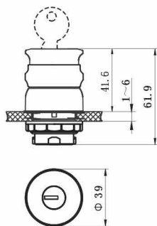
CZ4000-Y2E 防爆(急停)钥匙释放按钮操作头 CZ4000-Y2B 防爆(急停)钥匙释放按钮操作头 Operation head of explosion-proof (emergency stop) key-releasing push button
