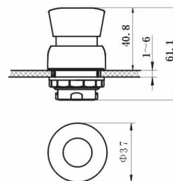
CZ4000-P4 防爆蘑菇头按钮操作头 Operation head of explosion-proof mushroom head push button
