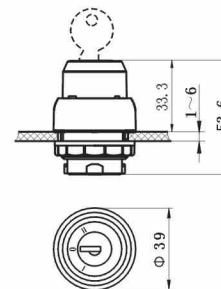
CZ4000-Y3 防爆钥匙按钮、开关操作头 CZ4000-Y8 防爆钥匙按钮、开关操作头 Operation head of explosion-proof key push button, switch
