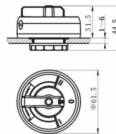
CZ4000-HE 防爆H四极开关操作头 CZ4000-HB 防爆H四极开关操作头 Operation head of explosion-proof H 4-pole switch
