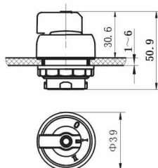
CZ4000-KB4 防爆开关操作头 CZ4000-KB8 防爆开关操作头 Operation head of explosion-proof switch
