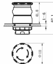
CZ4000-P6E 防爆(急停)扭动释放按钮操作头 CZ4000-P6B 防爆(急停)扭动释放按钮操作头 Operation head of explosion-proof (emergency stop) twist to release push button
